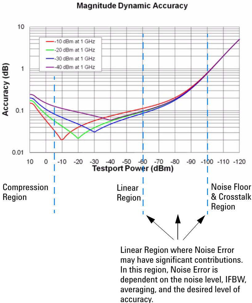
Figure 6 Receiver Magnitude Dynamic Accuracy
